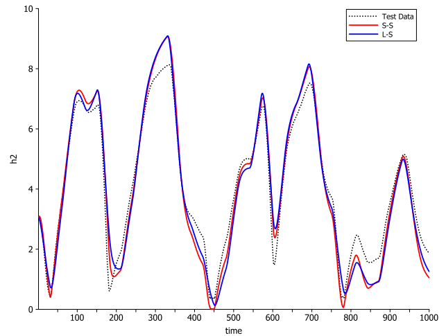
FIGURE 7. Simulation responses on the test data of the two top-ranked models S-S and L-S obtained from measured data.
