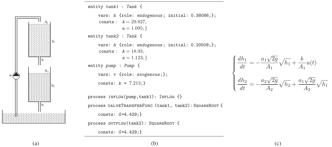
FIGURE 1. (a) The diagram of the three components of the water-tanks system; (b) The process-based model of the water-tanks system; (c) The equation-based model of the water-tanks system.
