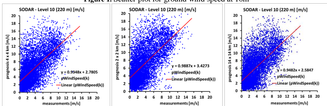
Figure 2. Scatter plot for wind speed at 220m (SODAR measurements)
