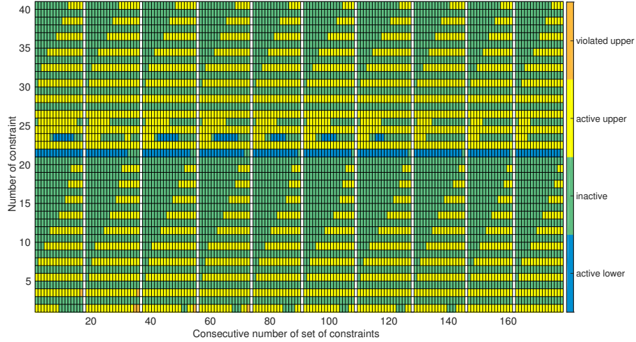
Fig. 1. Activity of constraints for the first 10 samples. The constraints are listed from the bottom to the top: the first 20 correspond to the soft constraints on \mathbf{x} from 1st to N -th time step within the prediction horizon, the following 20 are from constraints on \mathbf{u} for 10 steps and are hard. Samples are listed from left to right, the white columns separate blocks corresponding to different samples. For a given sample, the first list of active and violated constraints is in the leftmost column of the block and every change in the activity or violation during iterations results in a new column
