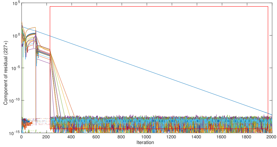
Fig. 4. The components of the dual residual \mathbf{d}^k from iteration 227 on (red frame) for sample 2 as a function of the iteration number
