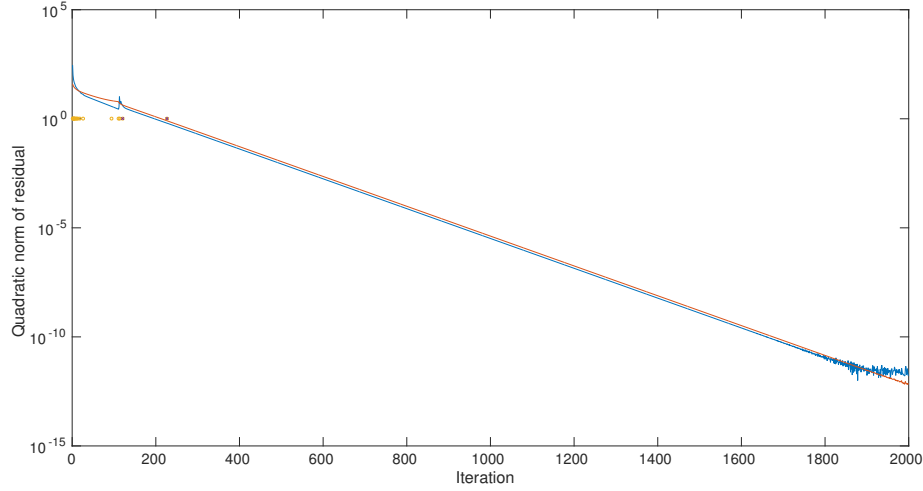
Fig. 2. Convergence of the quadratic norm of the primal (blue) and the dual (red) solution in sample 2 as a function of the iteration number. The yellow circles mark iterations in which the set of active constraints changes, the purple x's mark changes in the set of violated constraints
