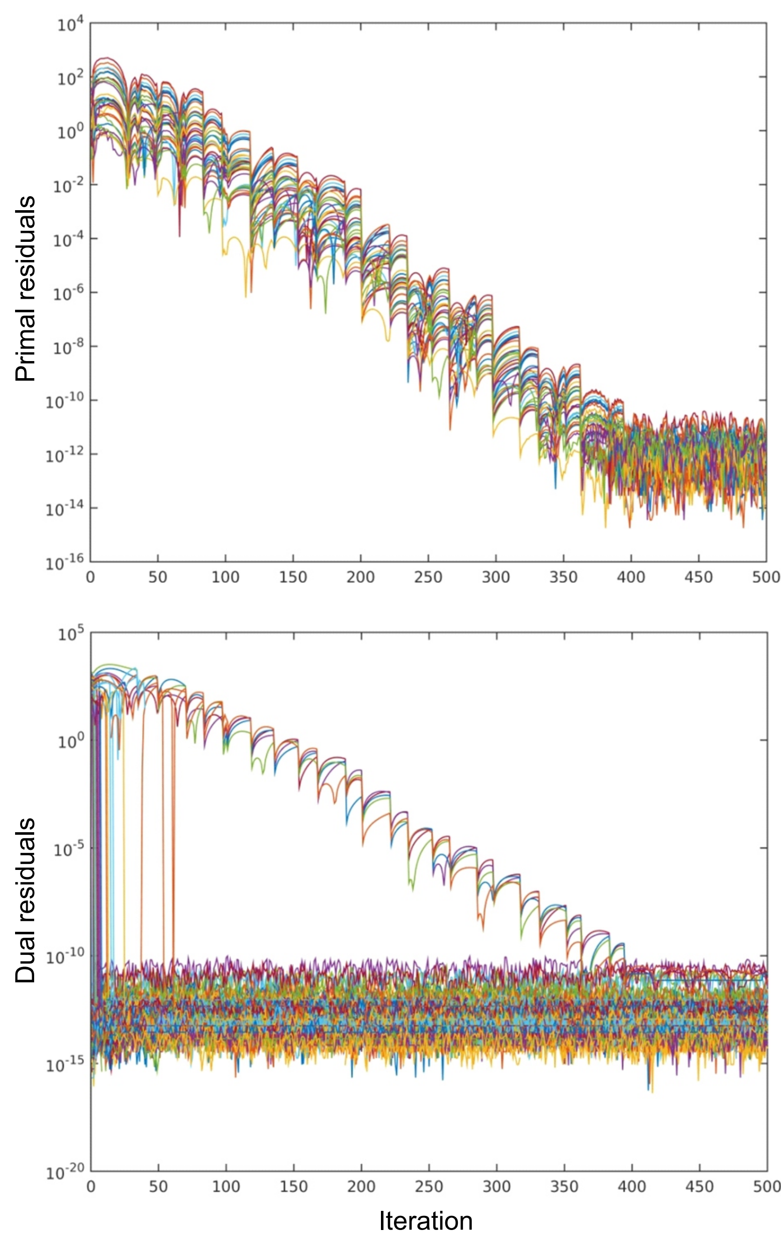
Example of convergence of primal and dual residuals in dFGM iterations for one time step of MPC
