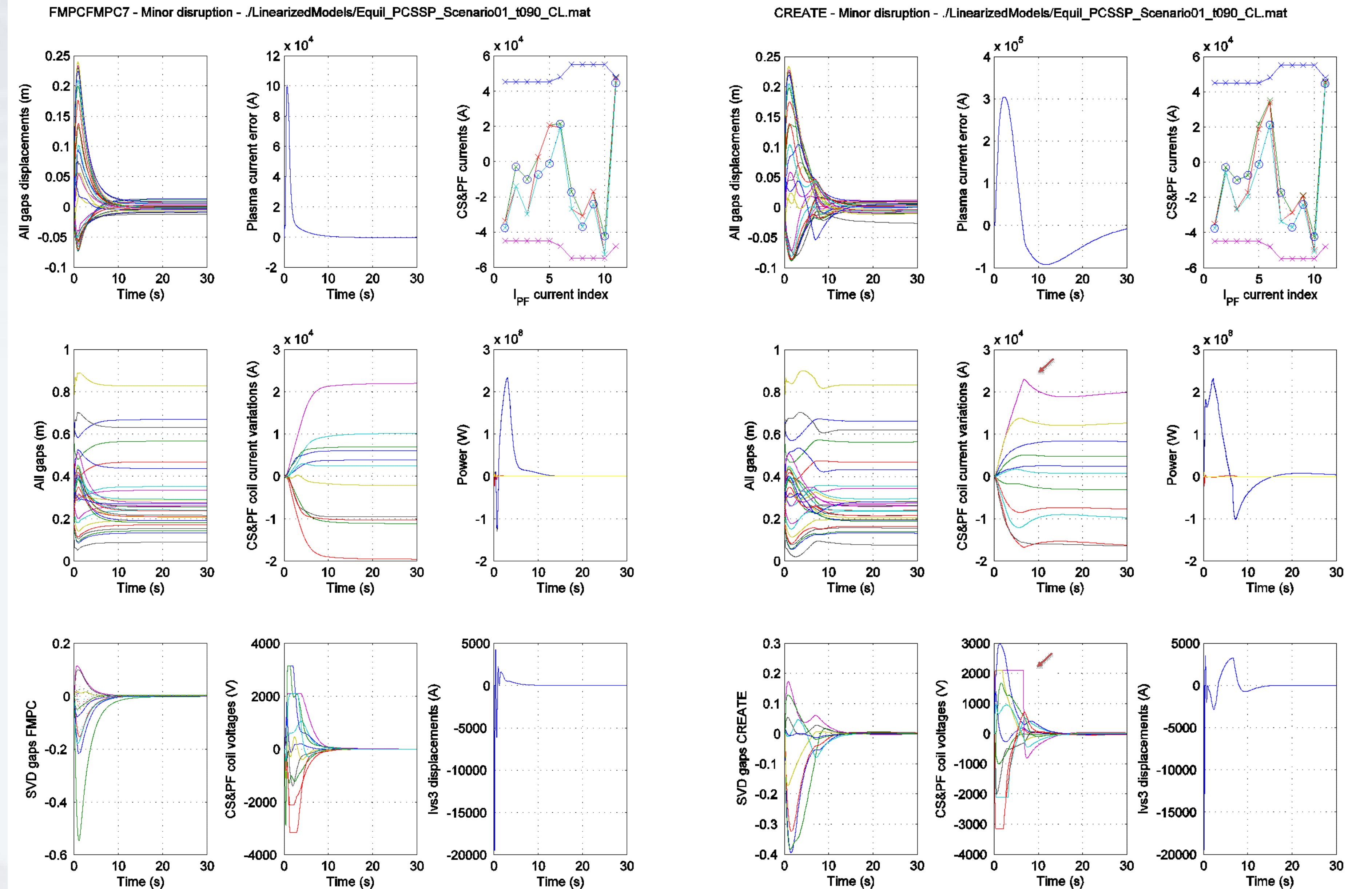
FMPC7-SVD PCSC: Minor Disruption, model t090
