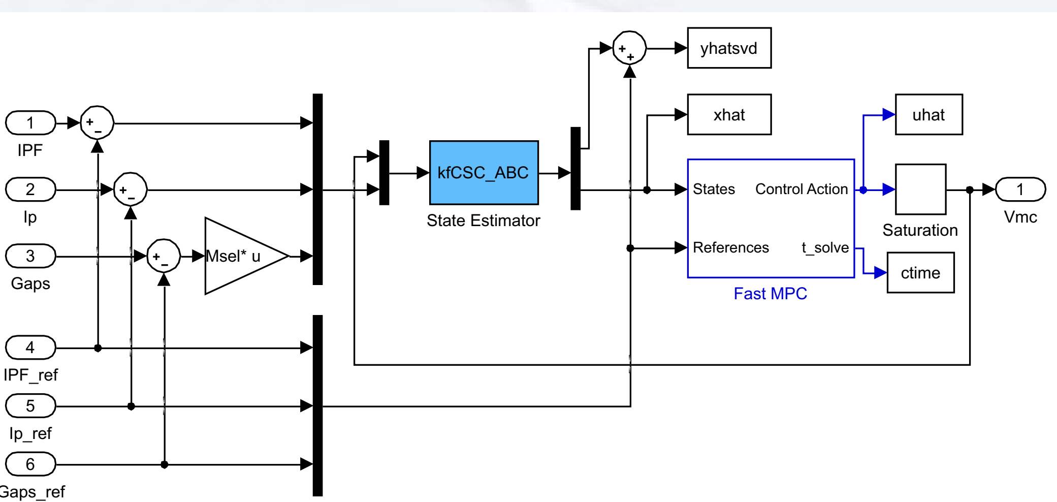
SVD-based fast MPC PCSC block scheme
