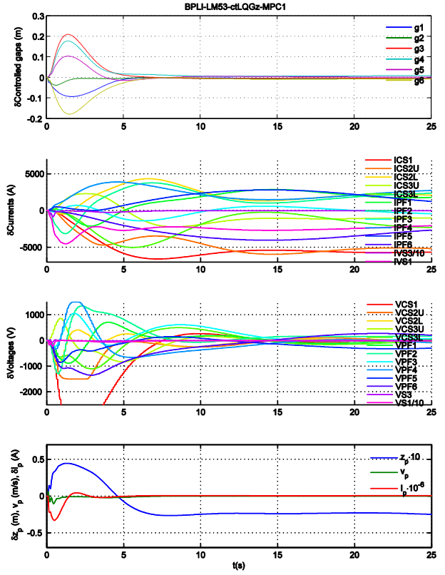
Fig. 3. BPLI simulation: ctLQGz-MPC, model LM53.
