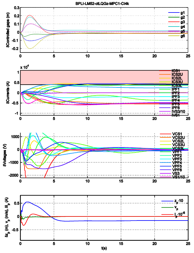
Fig. 7. BPLI simulation: ctLQGz-MPC, model LM52, with soft constraints \max(I_{pf}) \leq 4 kA.
