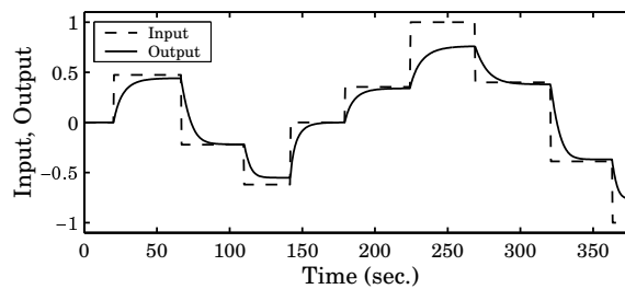
Fig. 4: Gain and time constant are non-linear functions of the operating point.
