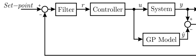
Fig. 3: General Internal Model Control Structure
