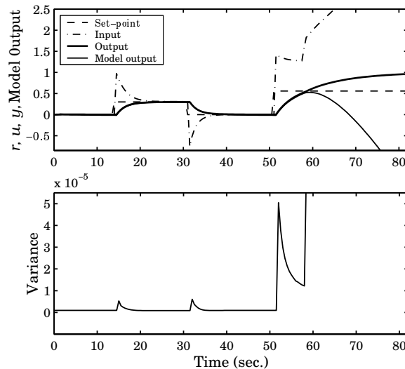
Fig. 6: Closed-loop response using Internal Model Control strategy. Desired closed-loop behavior was chosen as first order response, with unity gain and time constant of 2 seconds.
