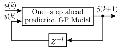
Fig. 5: Realisation of the parallel Gaussian Process model.
