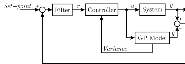
Fig. 7: Variance-constrained Internal Model Control Structure
