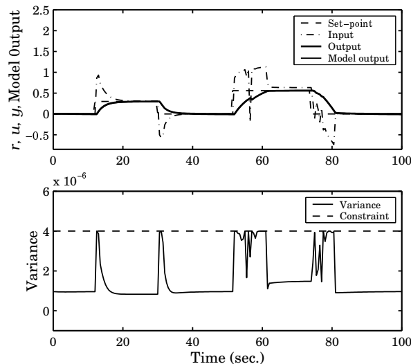
Fig. 8: Improved closed-loop response using variance-constrained Internal Model Control.
