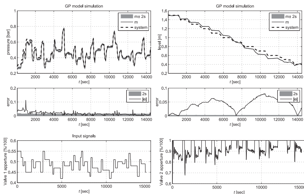
Fig. 2. Comparison of pressure measurement and Gaussian process model response (upper left figures), comparison of liquid level measurement and Gaussian process model response (upper right figures) and input signals into multi-input multi-output system (bottom figures)
